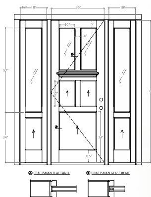
CAD Drawing
